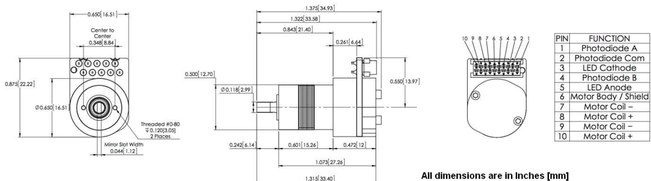
(Connector depicted above is TE Connectivity Micro-Match connector part number 8-215079-0.)
